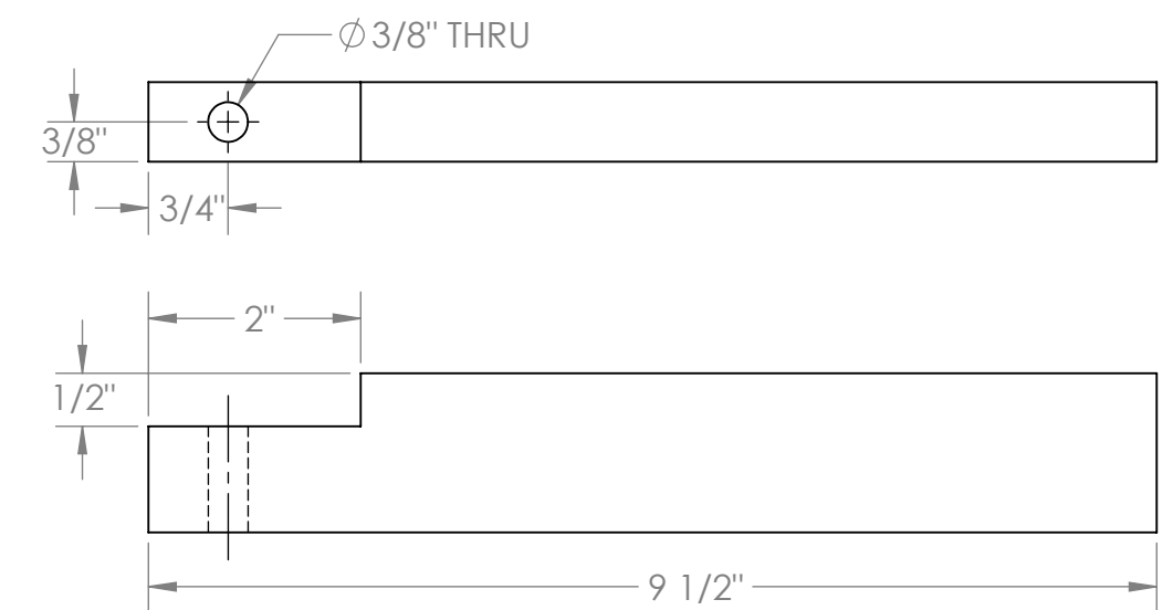
5 BOTTOM RAIL - OAK (1) REQUIRED
