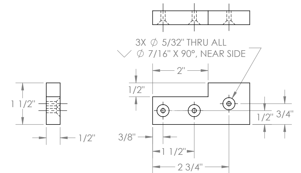
7 REINFORCEMENT PLATE, BOTTOM STRAP, W/HOLES - OAK (1) REQUIRED
