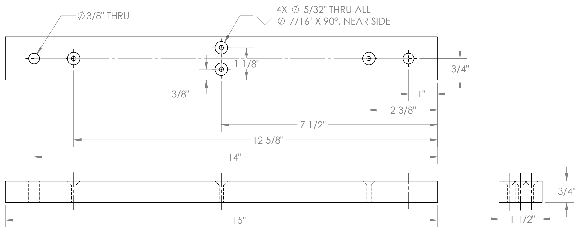
2 BOTTOM STRAP - OAK (2) REQUIRED
