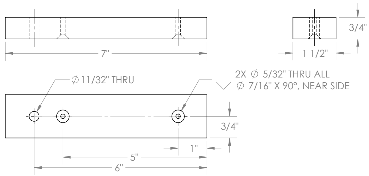
4 ARM STRAP - OAK (2) REQUIRED
