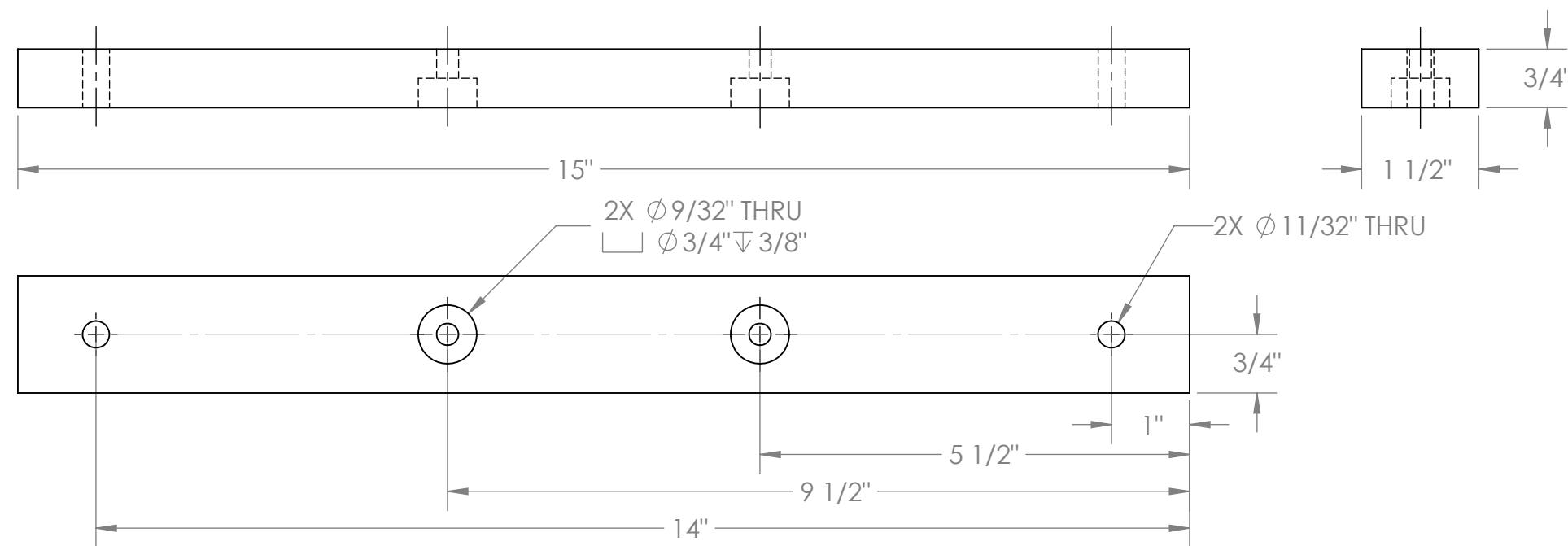
1 TOP STRAP - OAK (1) REQUIRED
