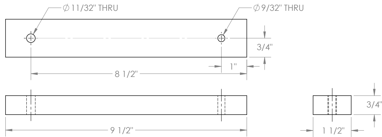
3 ARM - OAK (2) REQUIRED
