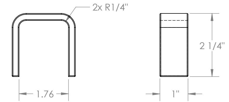
12 CLAMP BLOCK - FDM PRINTED - NYLON (1) REQUIRED
