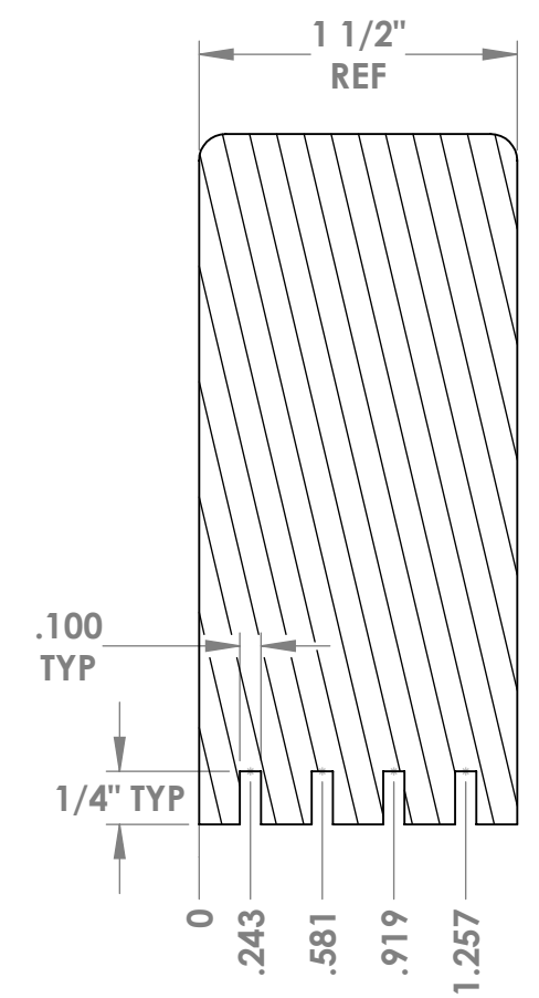
SECTION B-B
